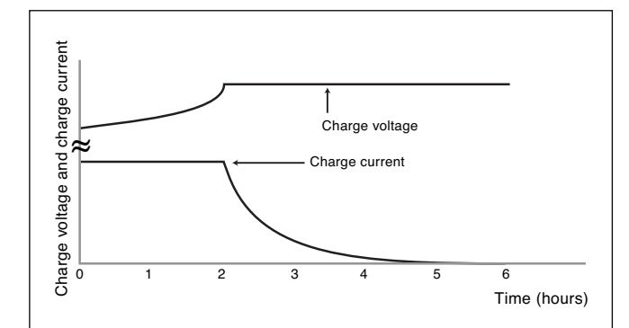
Constant voltage constant-current charge characteristics
