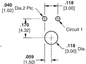
Recommended PC Board Layout 2 Position*
