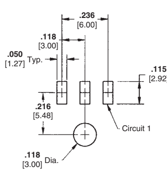
Recommended PC Board Layout * 3 Position
