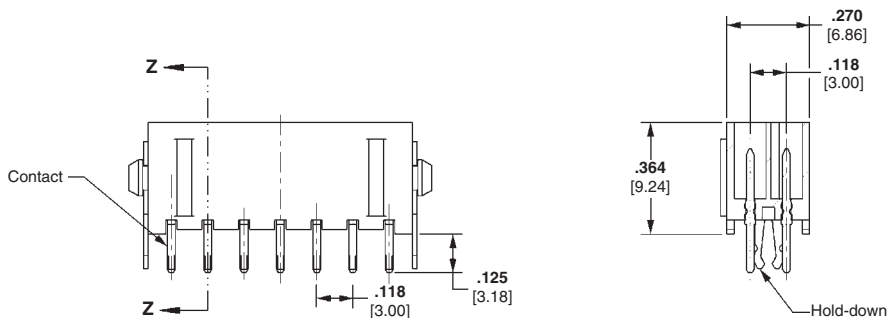
Section Z-Z
