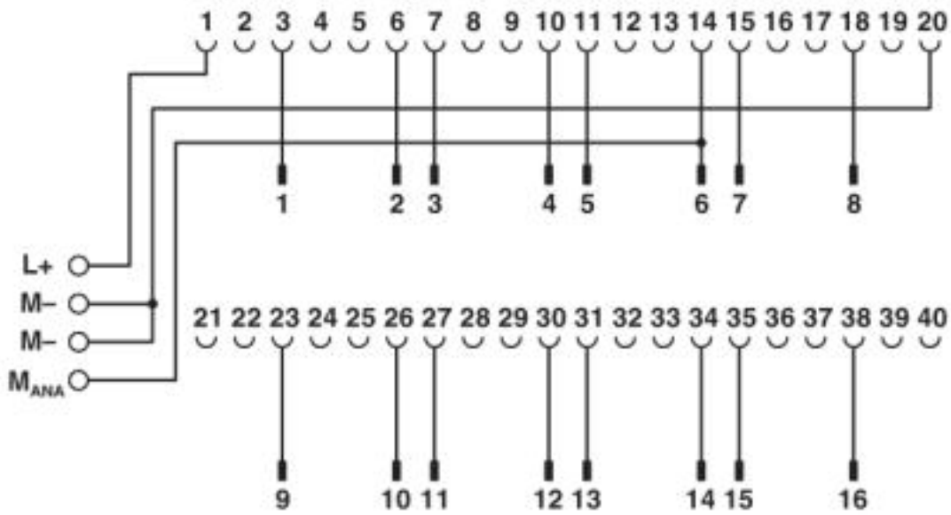
Connection scheme FLKM 16-PA-332-5HF//MINI-MCR
